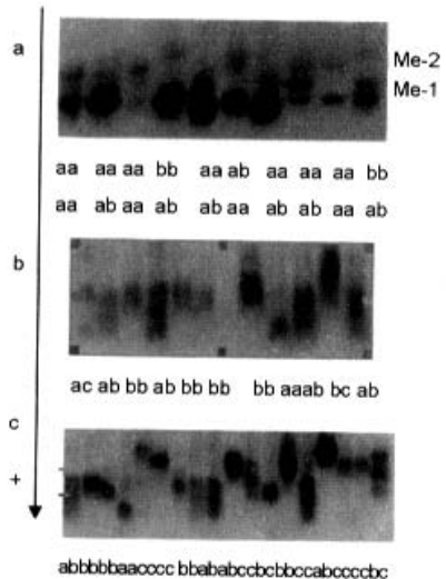
图2 同工酶电泳图谱 Fig.2 Diagram of isozyme electrophoresis a. Me; b. Sdh; c. Mdh
