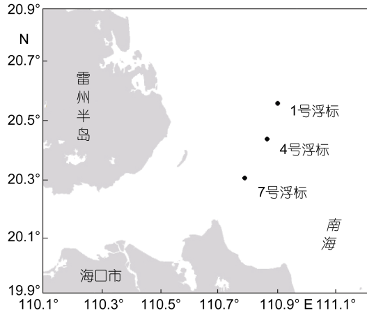
图1 雷州半岛东部近海浮标调查站位布设示意图 Fig.1 Location of the offshore buoys east of the Leizhou Peninsula, the northern South China Sea
